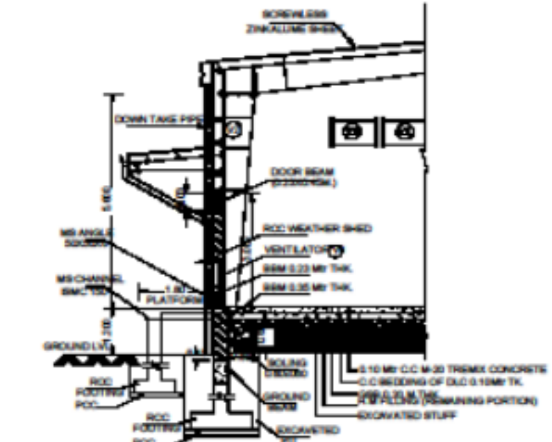
DETAILS OF FOOTING COLUMN BEAM PLATFORM TRUSS
