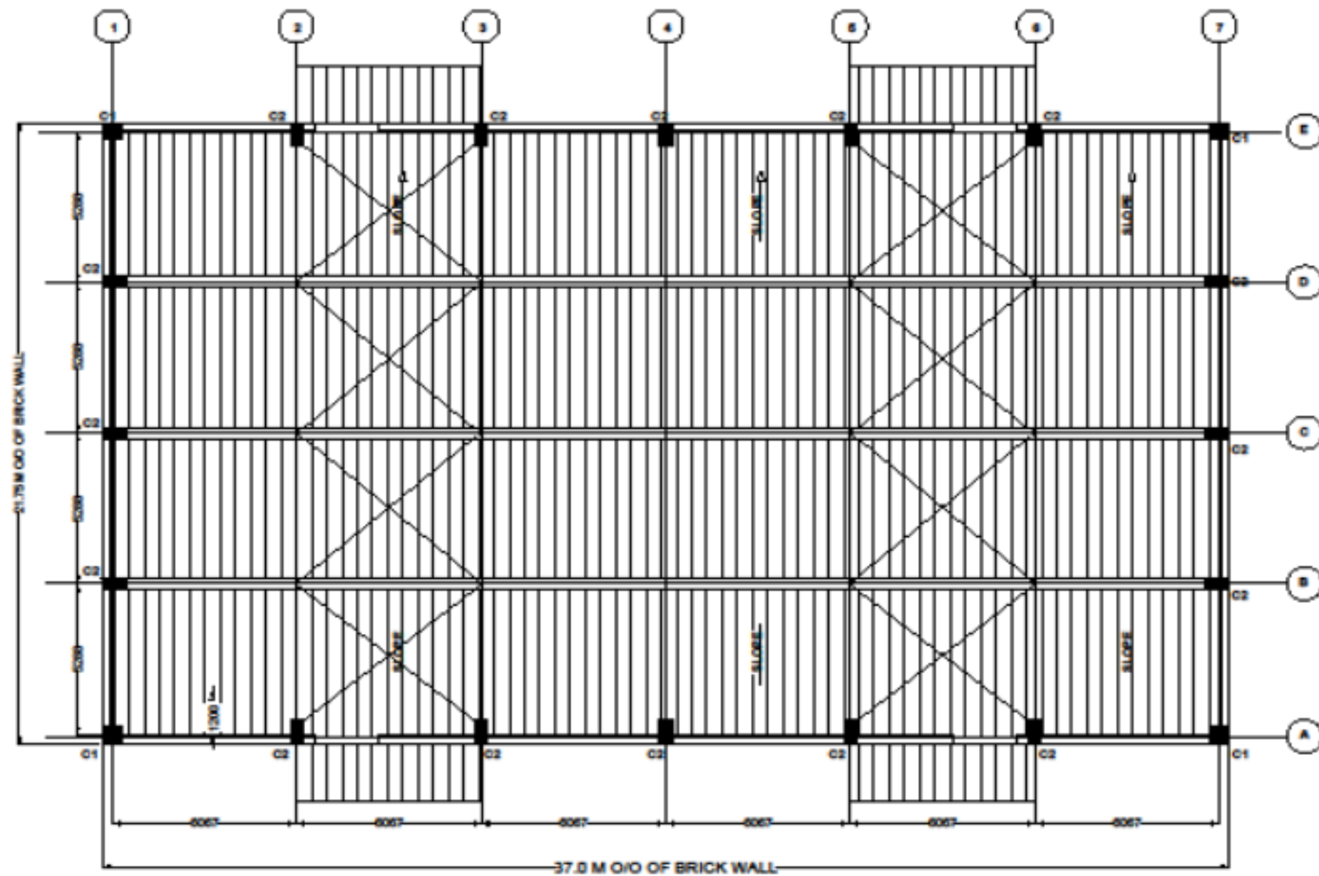
ROOF PLAN
