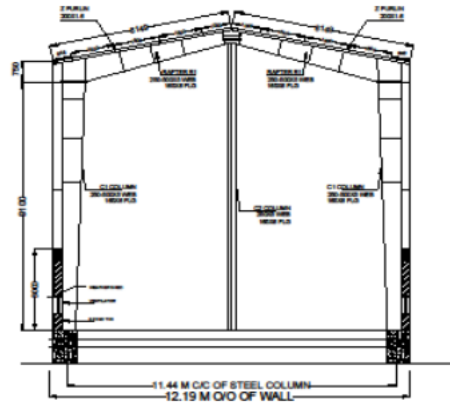
PORTAL FRAME AT 1 & 3
