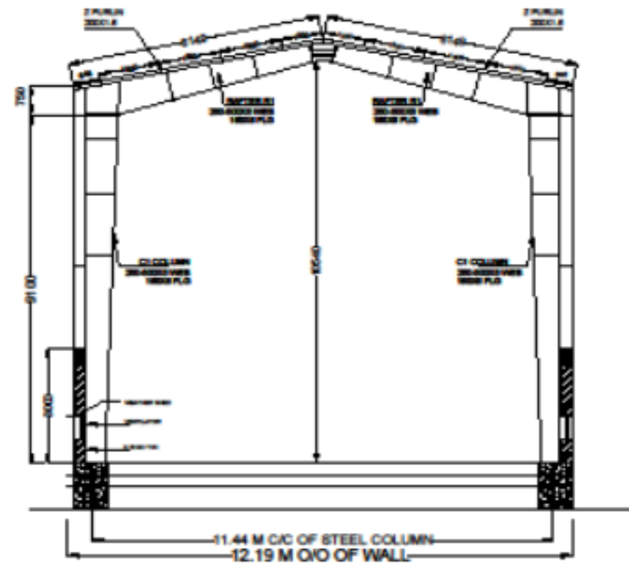
PORTAL FRAME AT 2
