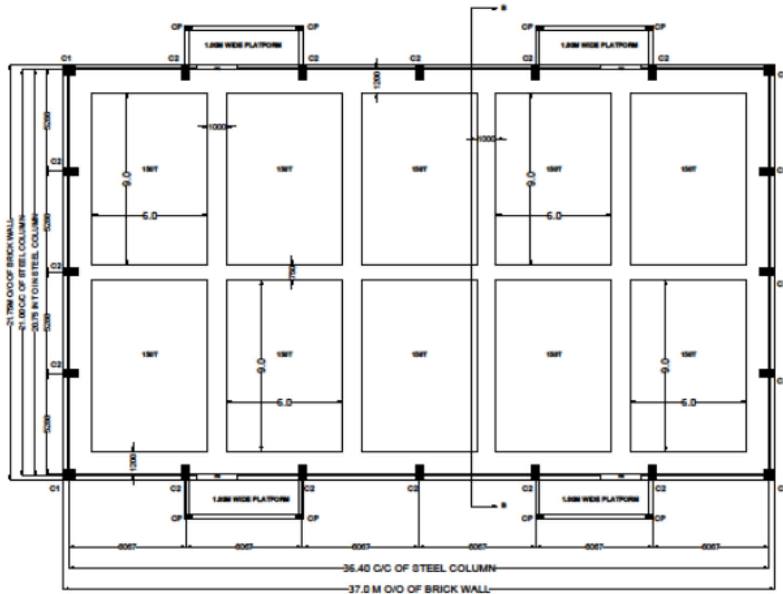
PLAN FOR 1/ 1500 MT WAREHOUSE BUILDING
