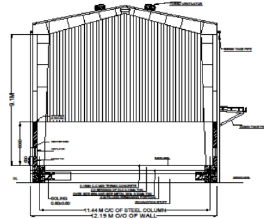
SECTION B-B
