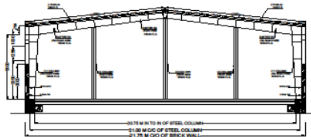
PORTAL FRAME AT 1 & 7
